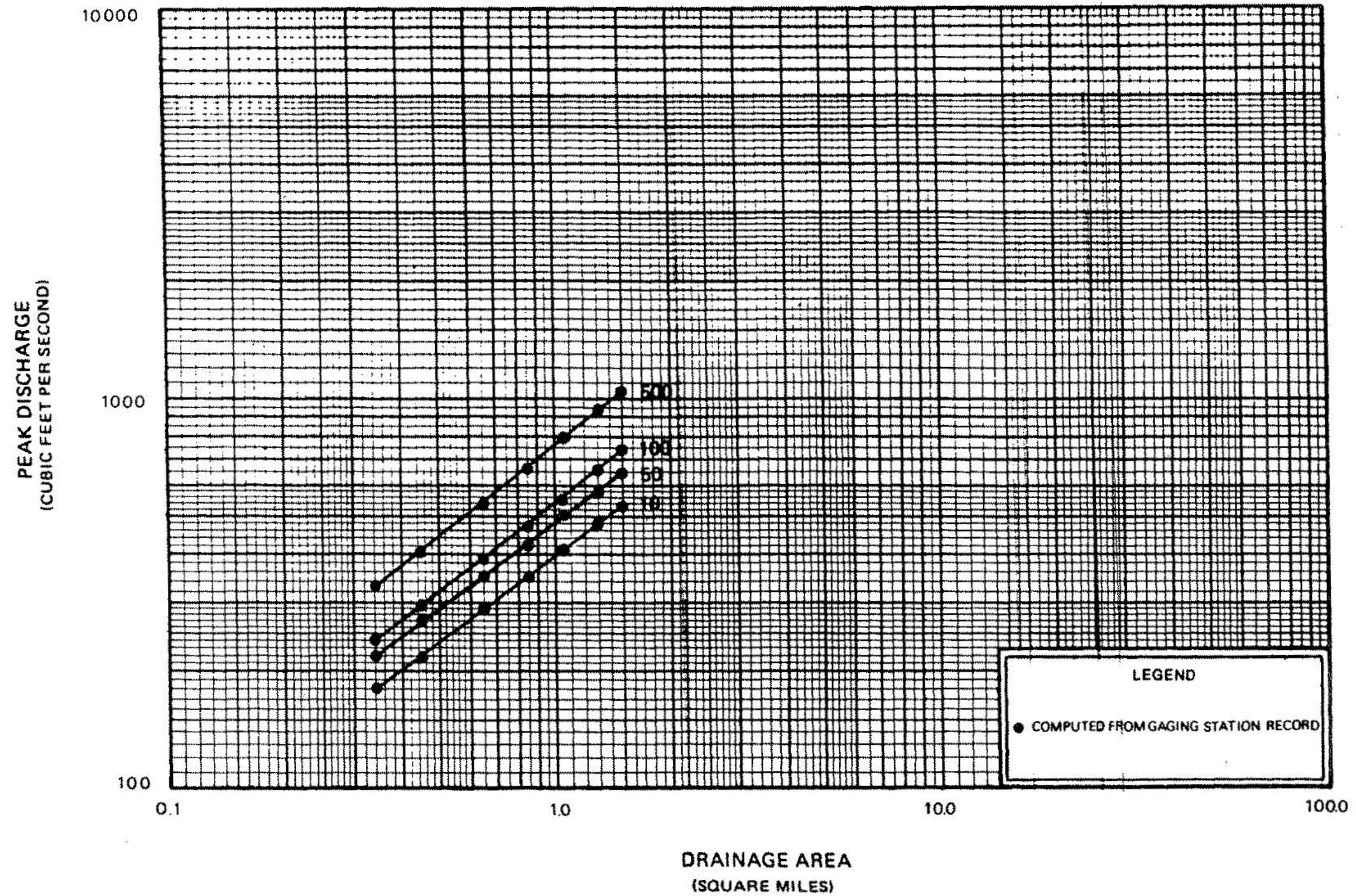
FIGURE 3 – FREQUENCY-DISCHARGE-DRAINAGE AREA CURVES – JENNING'S BROOK
