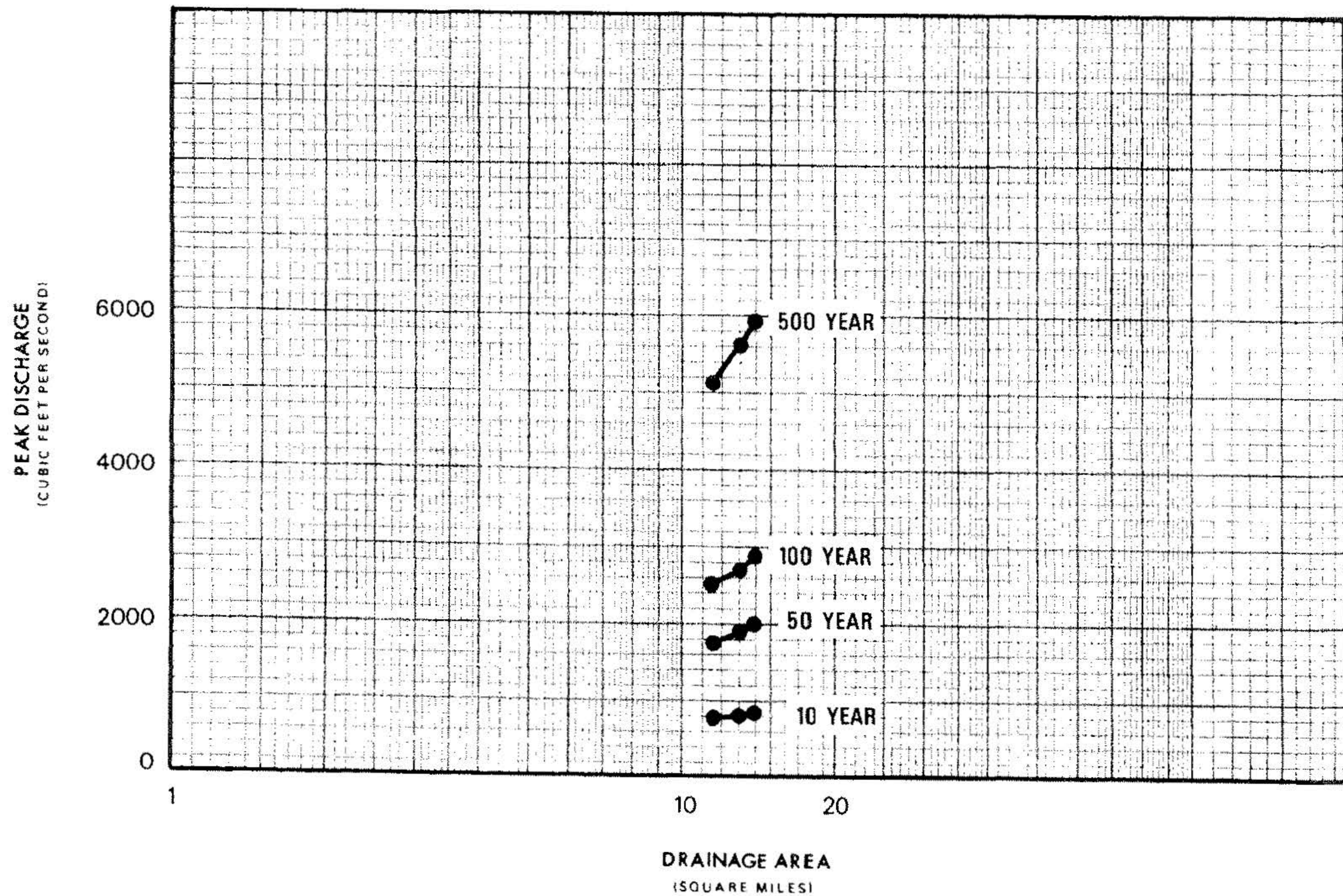
FIGURE 6 – FREQUENCY-DISCHARGE-DRAINAGE AREA CURVES – LIMEKILN BROOK
