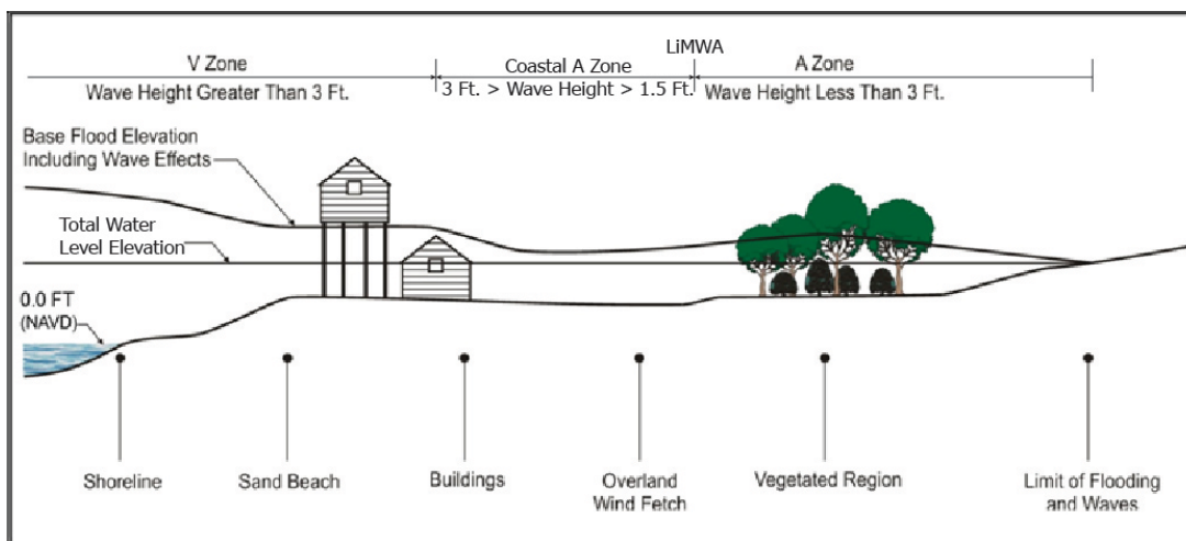
FIGURE 10 – TRANSECT SCHEMATIC
