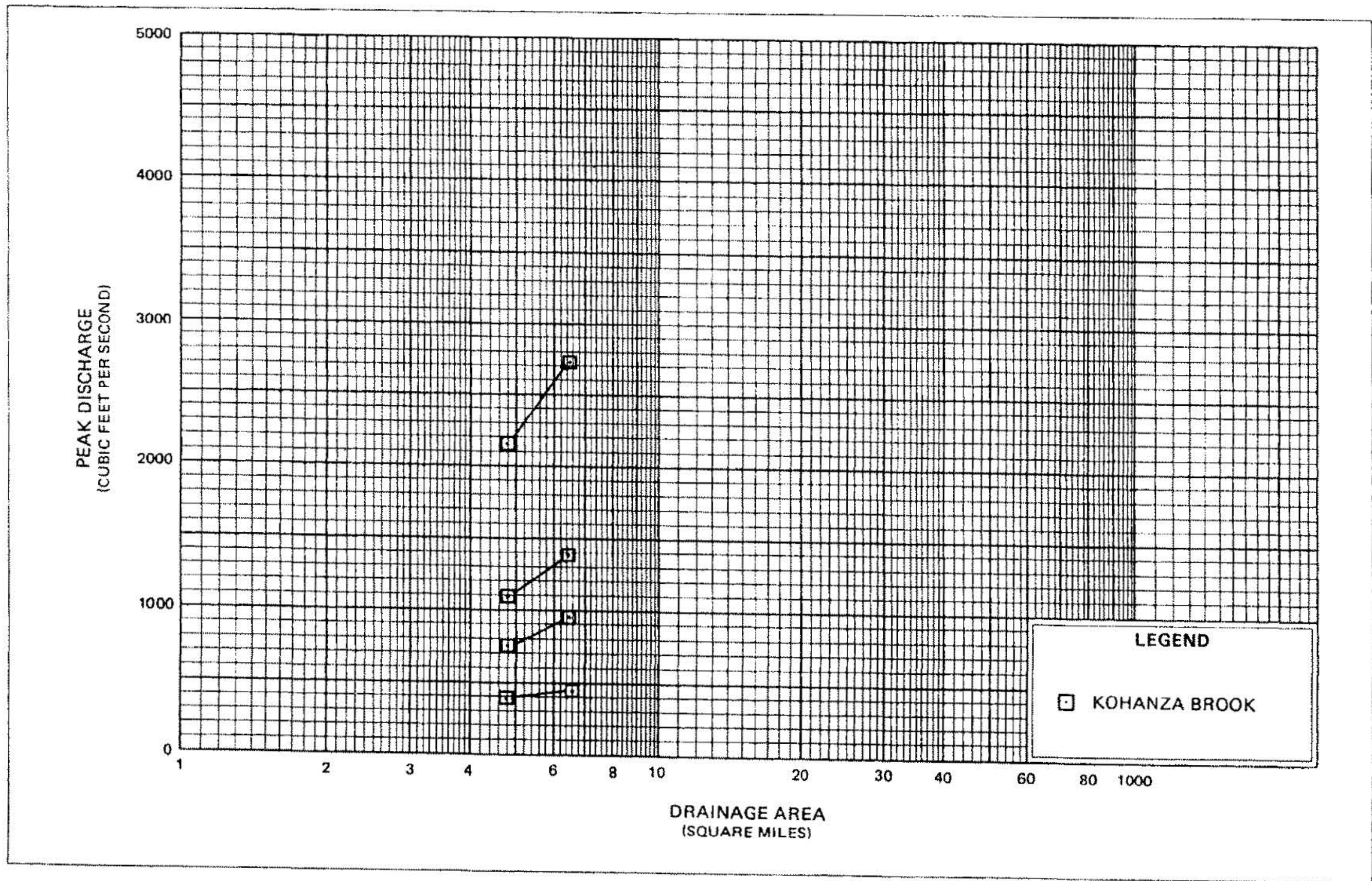
FIGURE 5 – FREQUENCY-DISCHARGE-DRAINAGE AREA CURVES – KOHANZA BROOK
