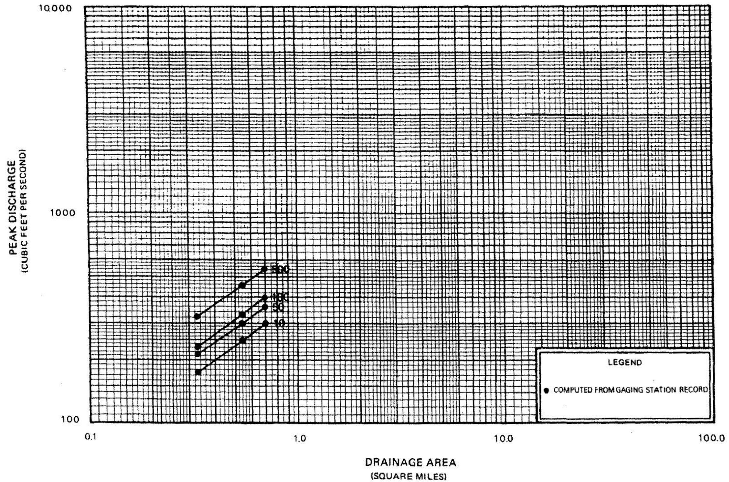
FIGURE 4 – FREQUENCY-DISCHARGE-DRAINAGE AREA CURVES – KETTLE CREEK
