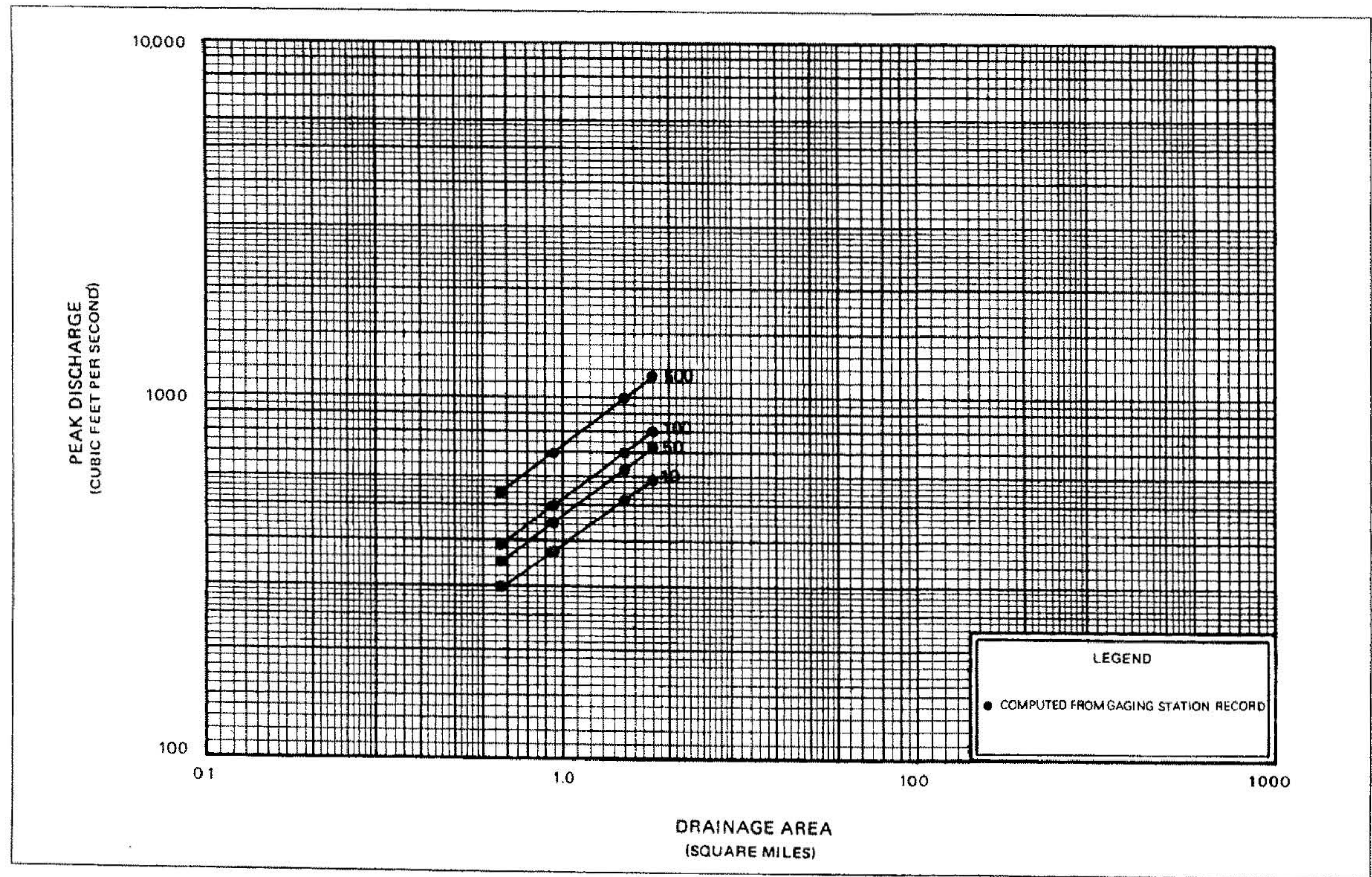
FIGURE 2 – FREQUENCY-DISCHARGE-DRAINAGE AREA CURVES – BEAVER BROOK
