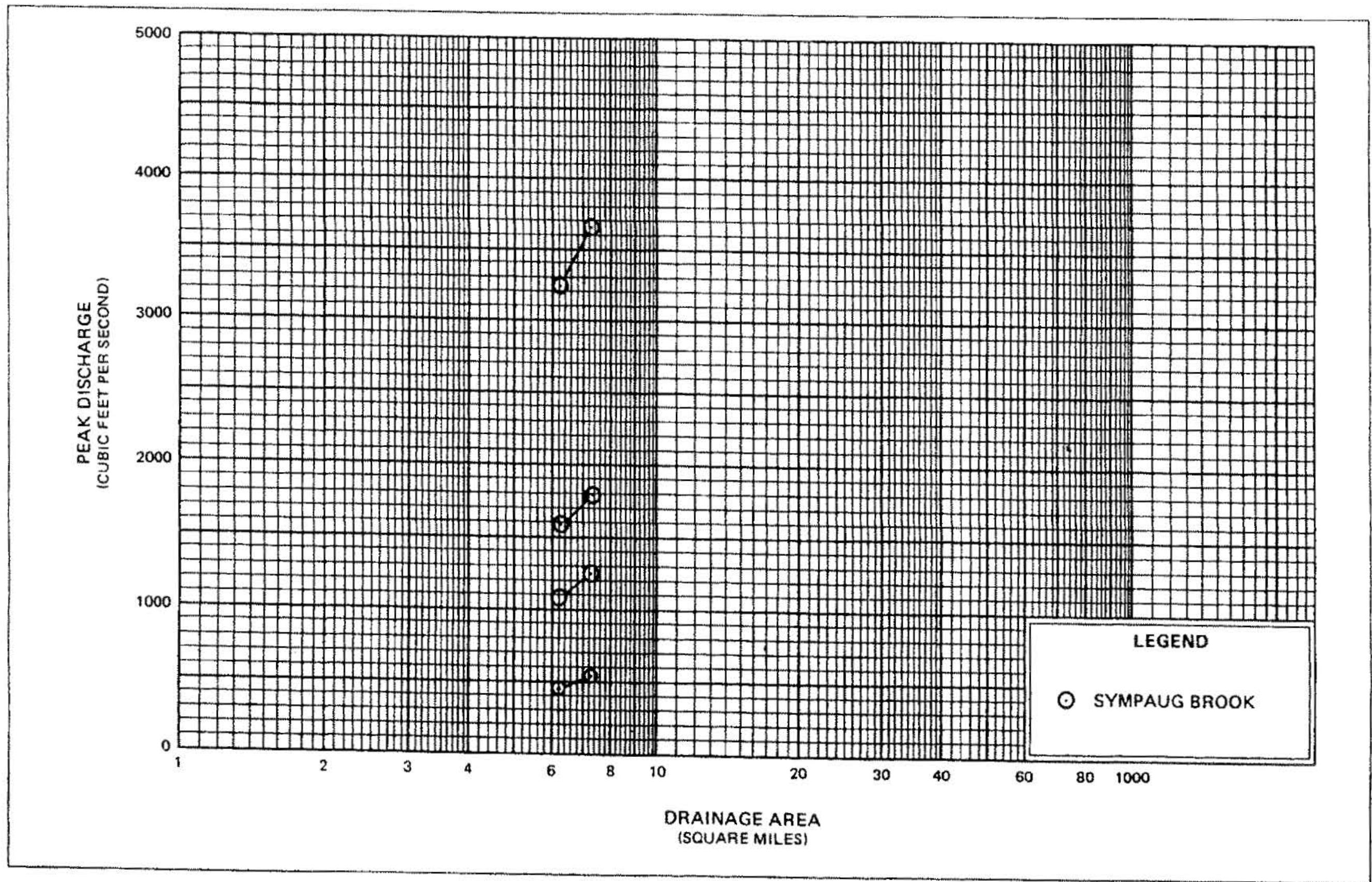
FIGURE 9 – FREQUENCY-DISCHARGE-DRAINAGE AREA CURVES – SYMPAUG BROOK
