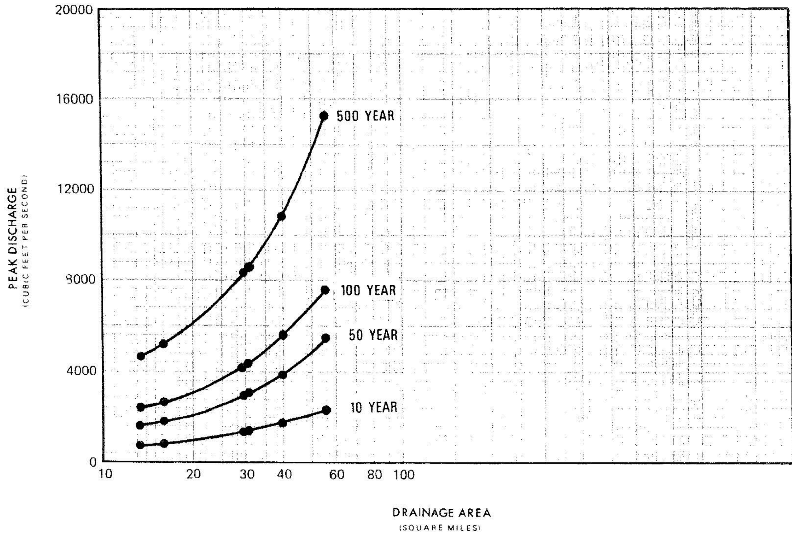
FIGURE 8 – FREQUENCY-DISCHARGE-DRAINAGE AREA CURVES – STILL RIVER
