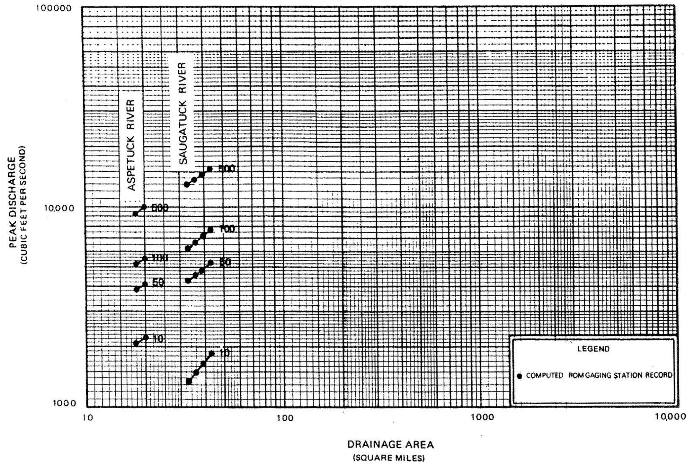
FIGURE 1 – FREQUENCY-DISCHARGE-DRAINAGE AREA CURVES – ASPETUCK RIVER (LOWER REACH) – SAUGATUCK RIVER (LOWER REACH) – SAUGATUCK RIVER (UPPER REACH)
