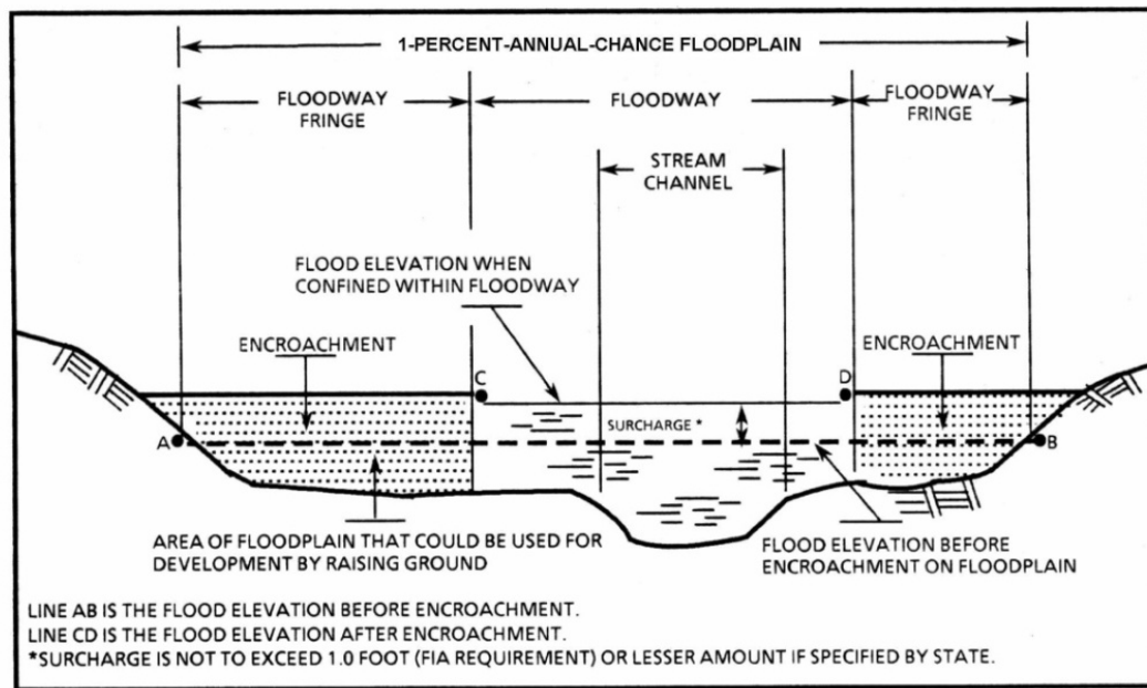
FIGURE 12 – FLOODWAY SCHEMATIC
